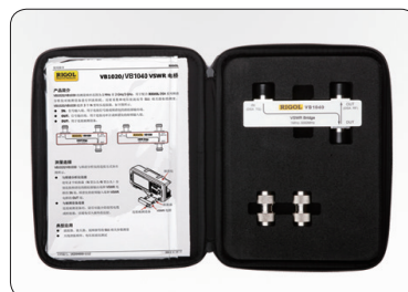
VSWR Bridge ( VB1032/VB1040/VB1080 )
