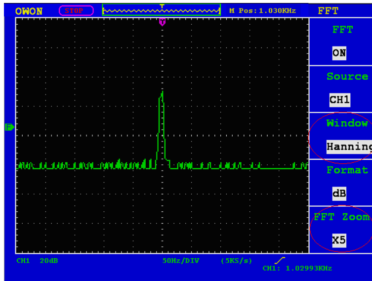
Fig.5-12 Hanning window
