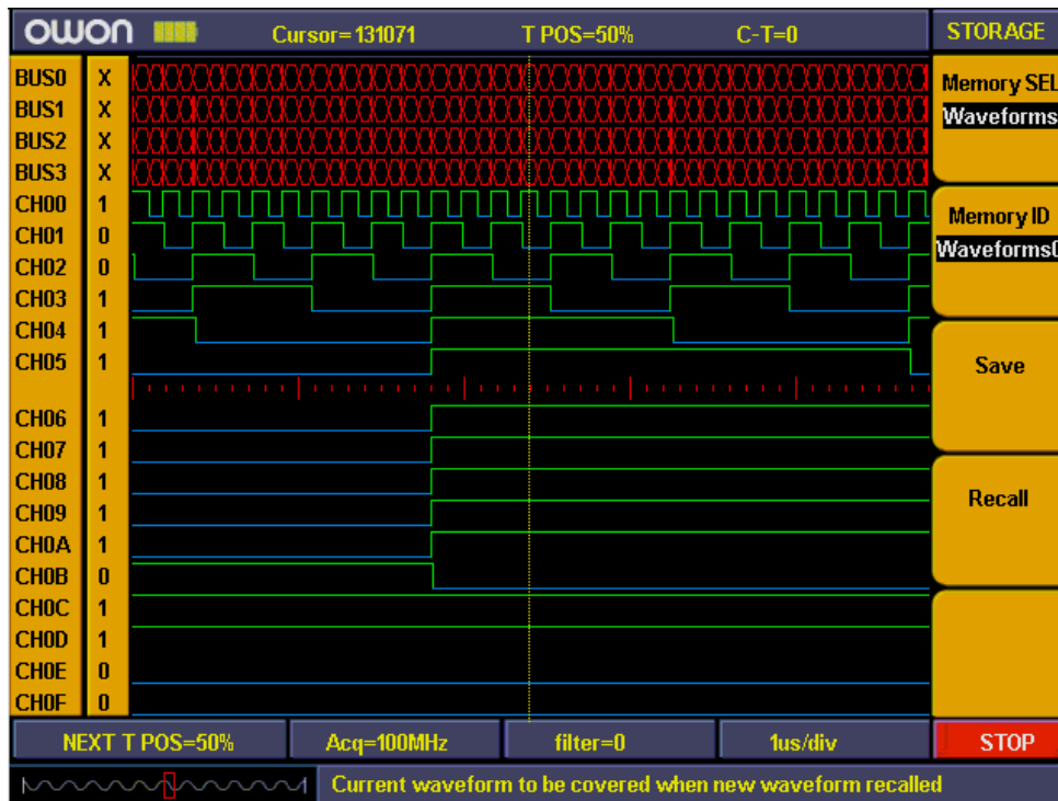
Fig.5-74: Waveform saving
