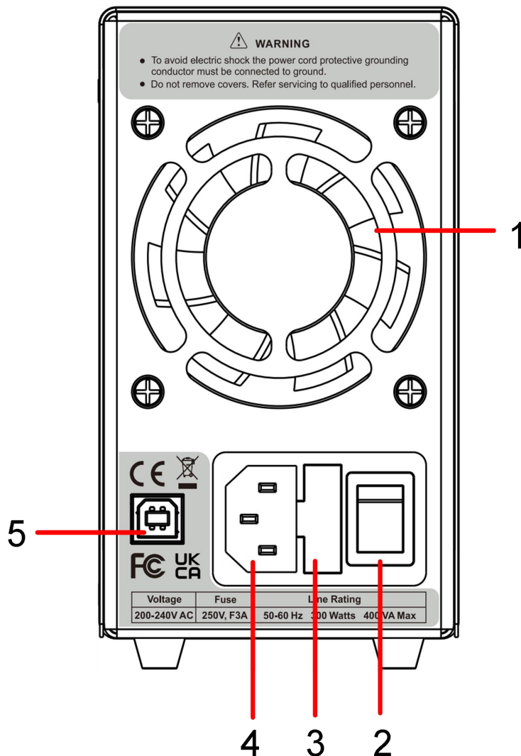
Figure 3-2 Rear Panel Overview
