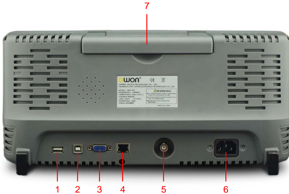
Figure 4-2 Rear Panel
