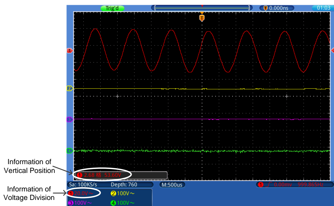
Figure 5-1 Vertical Information
