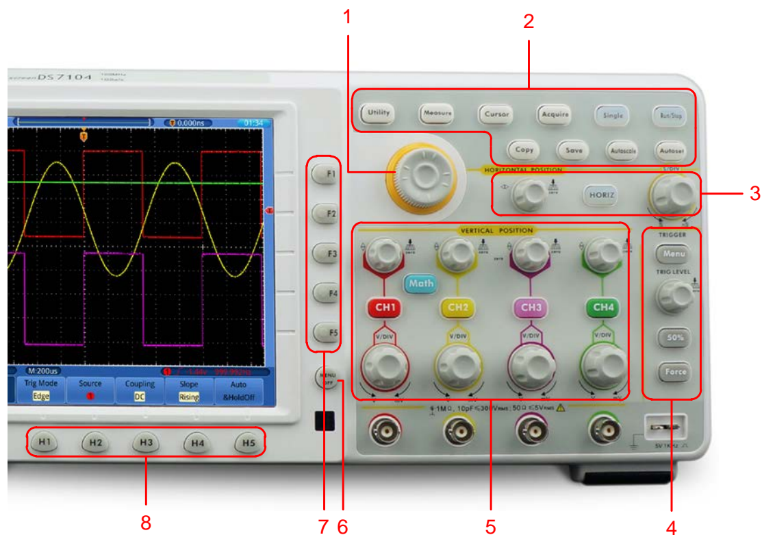
Figure 4-3 Keys Overview
