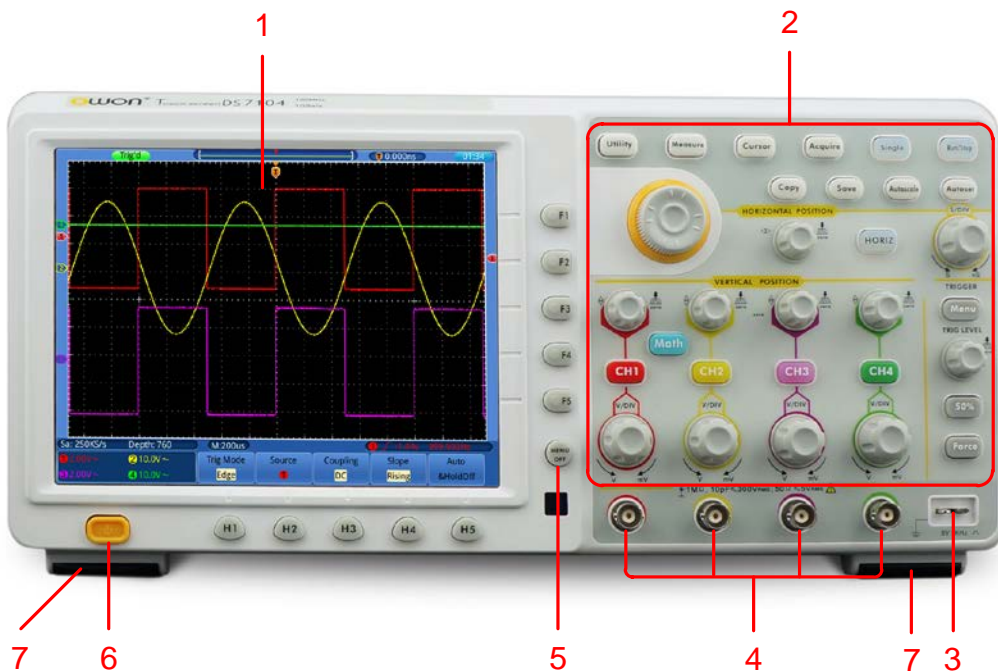
Figure 4-1 Front panel
