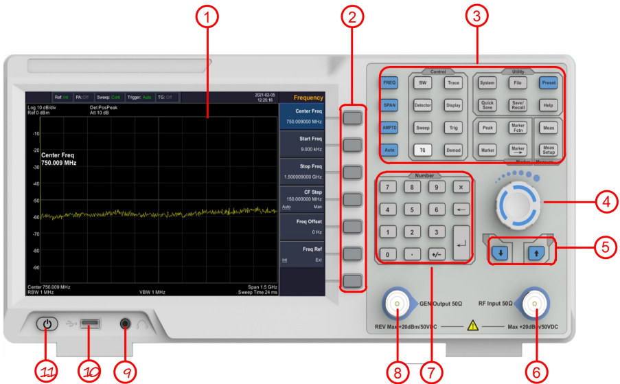
Figure 4- 1 Front panel
